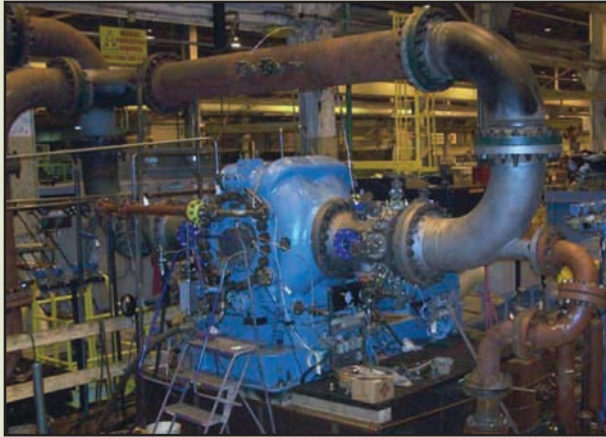
Figure 8. Experimental test rig.
