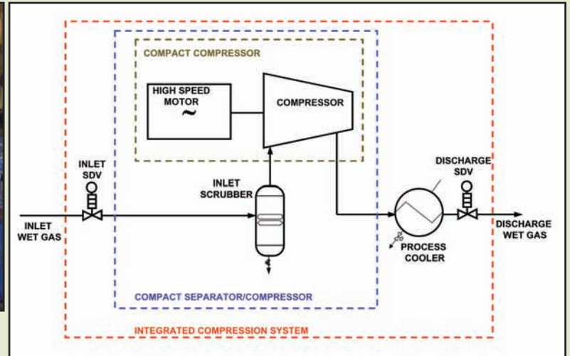
Figure 9. Schematic of single section compression process.
