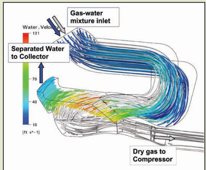
Figure 6. CFD modeling of rotary separator.
