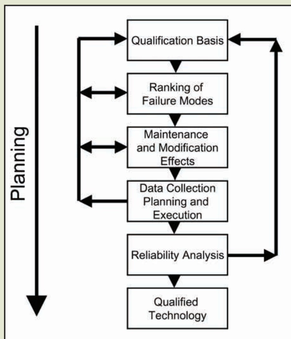
Figure 3. Schematic of main qualification activities. Ref. DNV-RP-A203 (2001).
