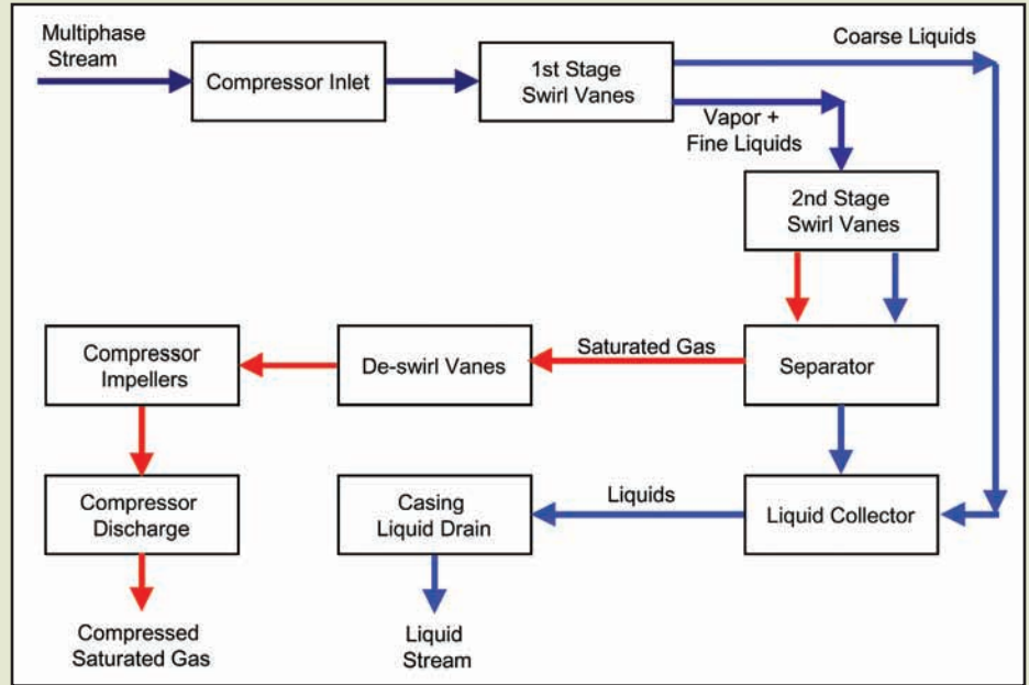
Figure 5. Main components of separator-compressor.
