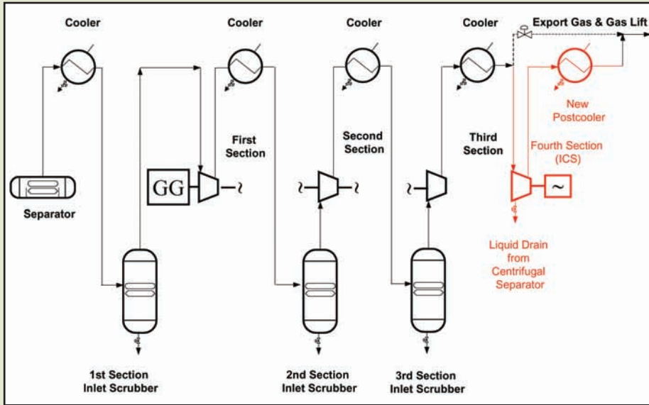
Figure 11. Integration of an ICS compression module into an existing platform.
