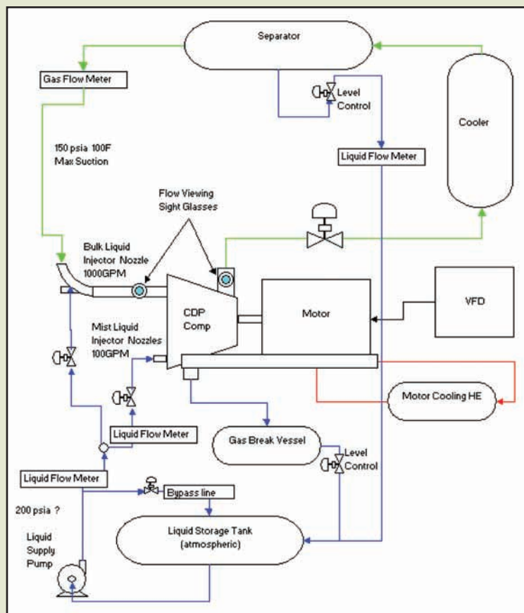
Figure 7. Schematic of multi-phase test loop.
