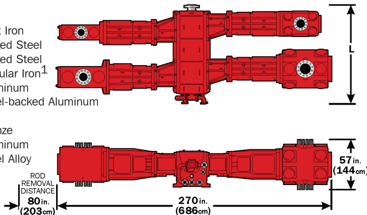
BDC-OF12H Typical Length (L) Dimension
